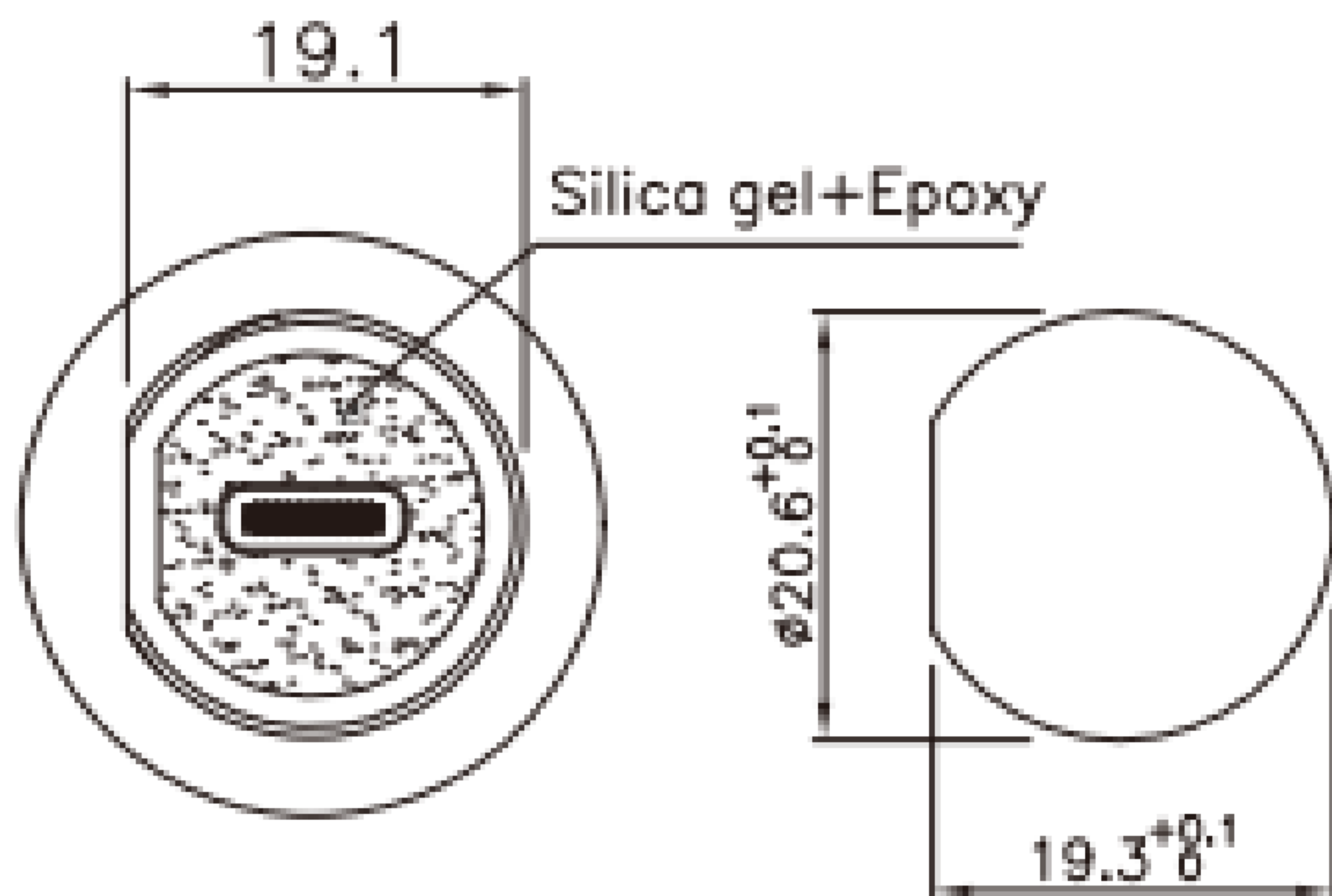
产品开孔尺寸 hole opening size
